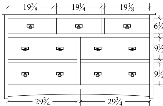
Dresser (OMDR66) 7 drawer 66w x 21 1/2d x 38h
