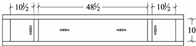
Storage Rail (3-2PLRQBRS)
