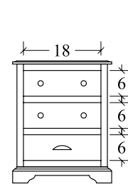
Night Stand (EANS3) 3 drawer 23w x 17d x 28 1/2h
