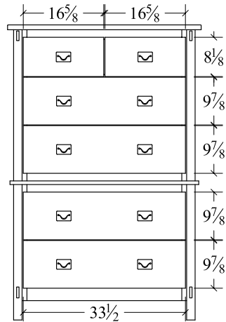
Chest on Chest (SHCDC) 6 drawer 40w x 22d x 61h
