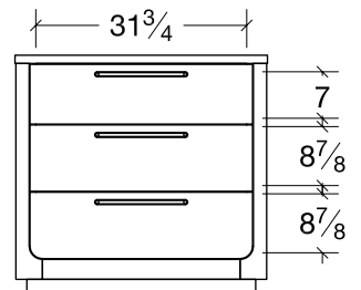
Chest (RSCD3) 3 drawer 38w x 18 1 / 8 d x 35 3 / 4 h
