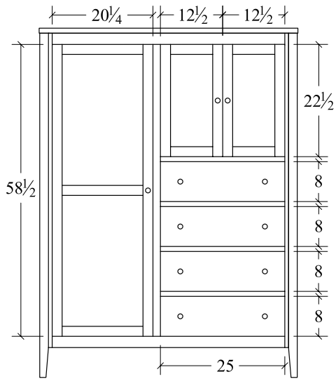
Chifferobe (HECB) 4 drawer, 3 door 1 shelf (behind small door) 3 shelves, 1 rod (behind large door) 52w x 21 1/2d x 70h
