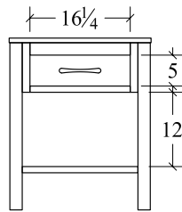
Nightstand (SBNS1) 1 drawer, 1 opening 23w x 17d x 27 3/4h
