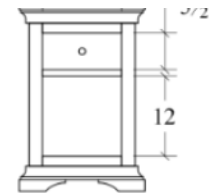
Nightstand (WTNS119) 1 drawer, 1 opening 19w x 16d x 28h
