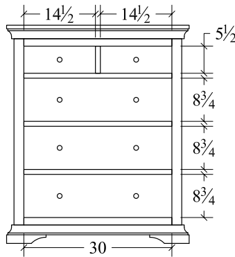
Chest (WTCD5) 5 drawer 37w x 22d x 44 1/4h
