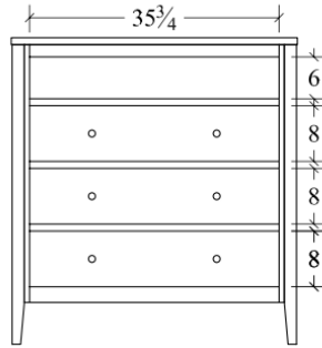
Media Chest (HEMC) 3 drawer, 1 opening 41w x 21 1/2d x 44h
