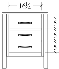
Nightstand (SBNS3) 3 drawer 23w x 17d x 27 3/4h
