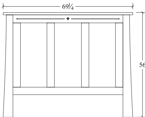
Queen Headboard 1-CAQB 69 1/4w x 56h
