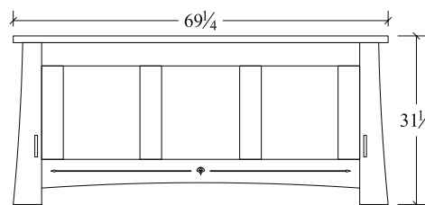
Queen Footboard 2-CAQB 69 1/4w x 31 1/4h
