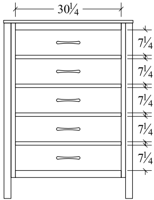
Chest (SBCD) 5 drawer 37w x 21 1/2d x 51h
